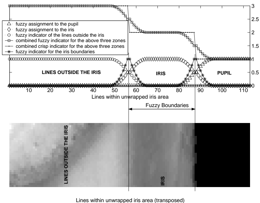
Figure 6: Fuzzy iris segment and fuzzy iris boundaries
